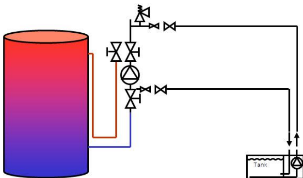
Standard Connection
