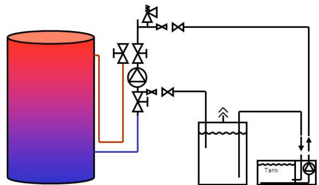
Connection w/Additional Reservoir
